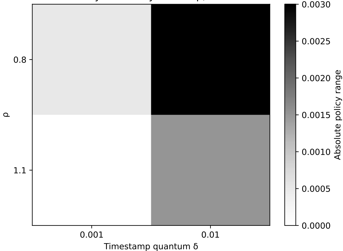
Policy sensitivity heatmap, K=1
