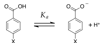
Figure 1: Acid equilibrium for benzoic acid
