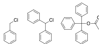
Figure 3: Benzyl chloride, diphenylmethylenes and triphenylmethyl acetate
