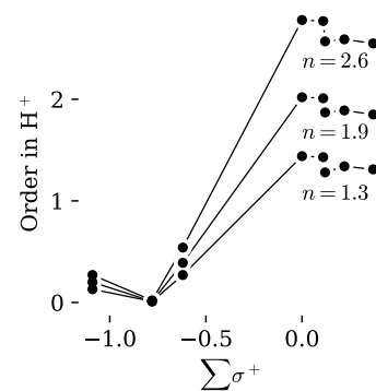
Figure 6: Plot of order of reaction in [\text{H}^+] ( n ) vs \Sigma \sigma^+ using three different sets of H_0 values.
