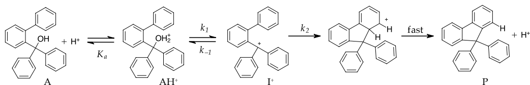
Figure 3: The full proposed mechanism of the reaction.
