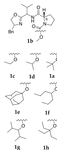
Figure 5: The ligand series explored in the paper. 1 ↓
