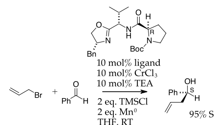
Figure 5: The ligand series explored in the paper. 1 ↓
