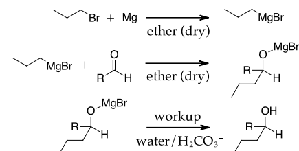
Figure 1: A Grignard reaction.↓
