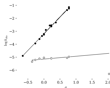
Figure 4: The same plot as in figure 3 with the value for ortho -nitrobenzoate included.
