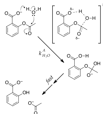
Figure 5: Proposed mechanism #1: intramolecular general base catalysis. ↓
