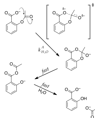
Figure 6: Proposed mechanism #2: anchimeric assistance by carboxylate. ↓
