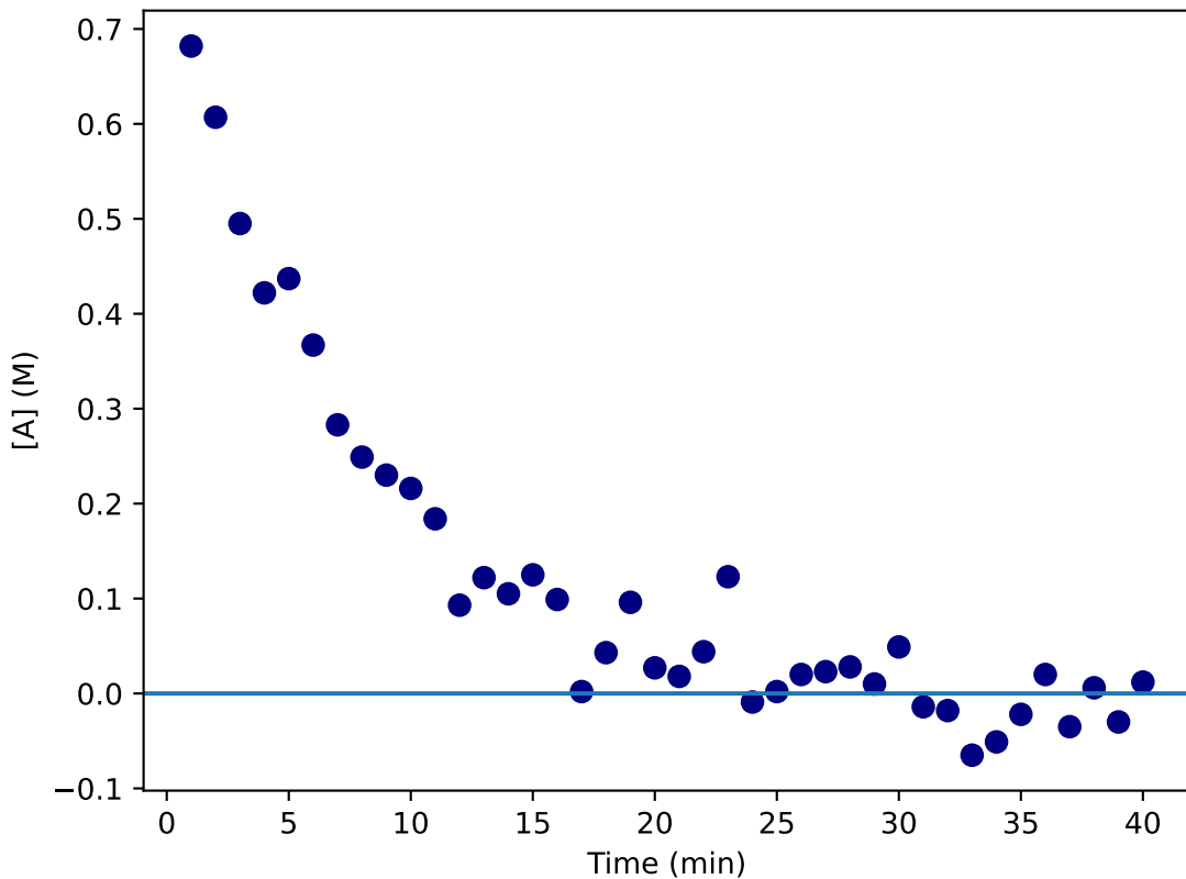
Simulated First-Order Kinetics
