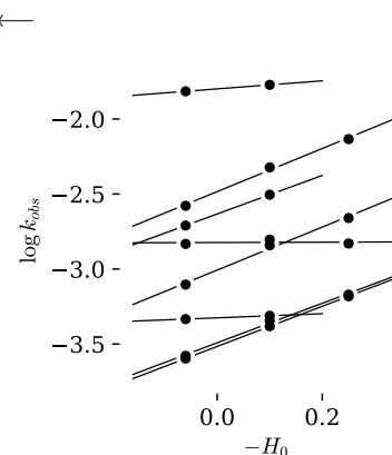
Figure 5: Plot of k_{obs} vs H_0 for a series of reactants.
