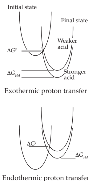
Figure 1: Marcus analysis of reaction coordinates for two cases of general acid catalysis. Equation 1: The Brønsted equations for acid and base catalysis.
