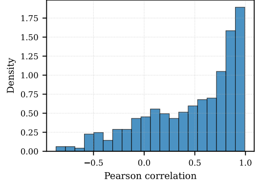
Figure 9: Pearson correlation distribution between rollout score sets from the external RM (sfairXC/FsfairX-LLaMA3-RM-v0.1) and our contrastive self-judge score. The mass near 1 indicates strong but not complete agreement.
