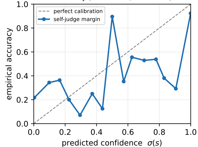
Reliability (Brier 0.198, ECE 0.294)
