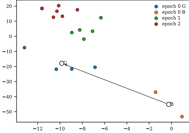
Figure 7: PCA projection of Qwen3-8B generations (embedded with Qwen/Qwen3-Embedding-4B) on an AlpacaEval prompt: points move from the B group toward the G group after the first iteration; later iterations refine the direction as guidance updates.
