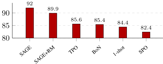
Llama3-8B-Instruct
