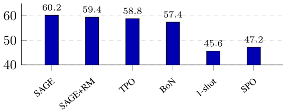
Llama3-8B-Instruct
