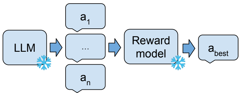
Test time alignment methods with RM
