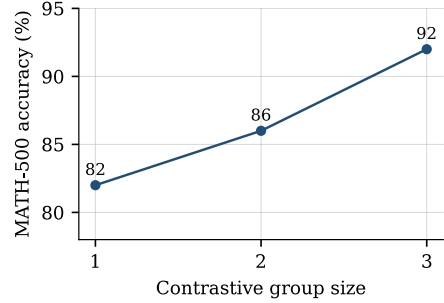
Figure 9: Symmetric cap on the sizes of the good and bad groups (the k best and k worst candidates enter the gradient step) vs. MATH-500 accuracy on a 50-problem subset (Qwen3-8B); the point at 3 corresponds to the default asymmetric 4-good/3-bad configuration. Larger groups yield better textual gradients than extreme-only (best-versus-worst) feedback. The full-benchmark headline is reported in Table 1.
