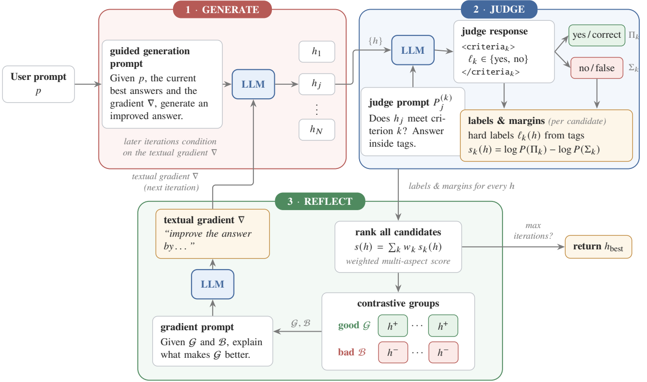
Figure 2: The SAGE framework: a single LLM acts as generator, self-judge, and reflector. Candidates are scored with contrastive label margins, partitioned into good and bad groups, and a textual gradient \nabla extracted from the groups guides the next generation round.
