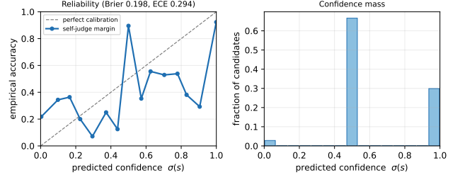
Figure 11: Reliability diagram (left) and confidence-mass histogram (right) for the self-judge margin over all MATH-500 candidates, pooled across three seeds. The margin ranks correct above incorrect candidates (selection AUC 0.64) but is over-confident as an absolute probability ( \text{ECE}_{15} = 0.294 ), matching our use of it purely as a selection/grouping signal.
