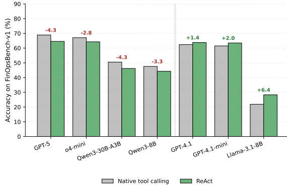
Figure 6: Native tool calling vs. ReAct on FinOpsBench-v1. Numbers above each pair give the ReAct minus Native delta in percentage points.
