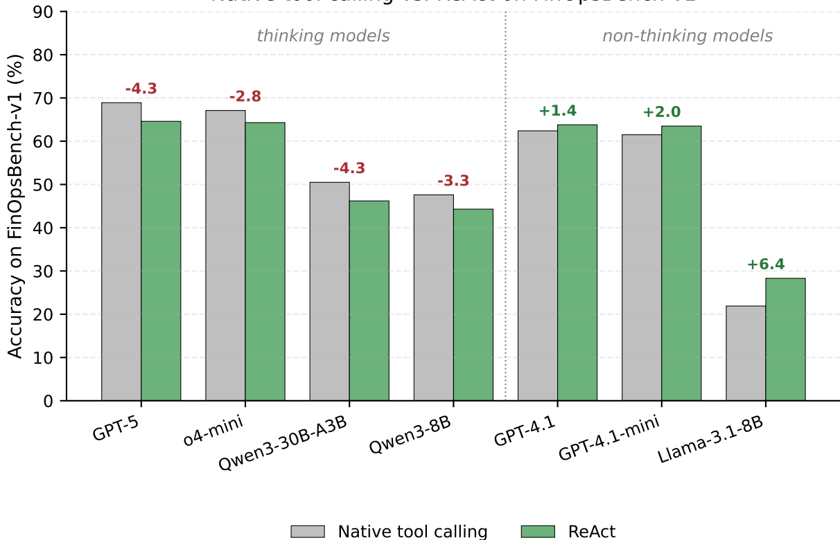
Native tool calling vs. ReAct on FinOpsBench-v1
