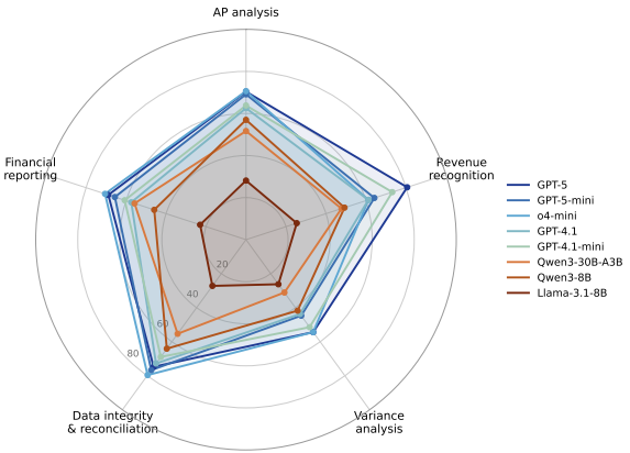
Figure 6: Per-category accuracy on FinOpsBench-v1 for the eight evaluated models. Axes are the five categories described in Section 3.2; each query in the 729-example test set is assigned to one of these five categories. The category mix of the full FinOpsBench-v1stream is reported in Appendix G.
