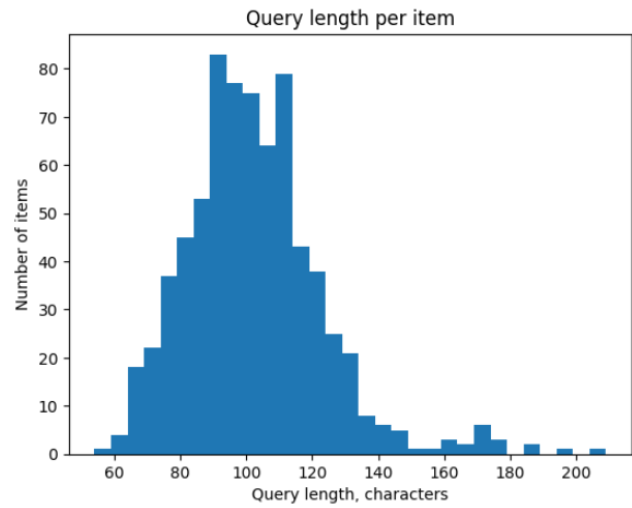
Figure 10: FinOpsBench-v1: Query length distribution.
