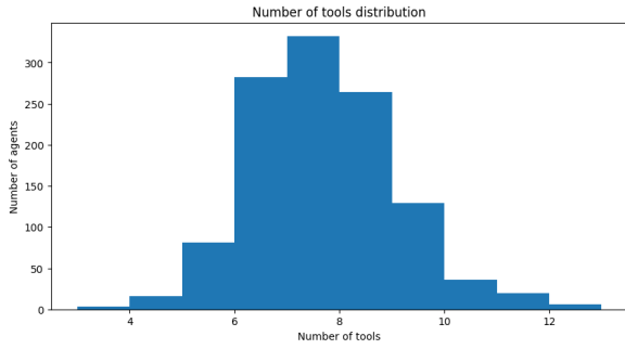
Figure 18: FinOpsBench-v2: Number of tools per example.
