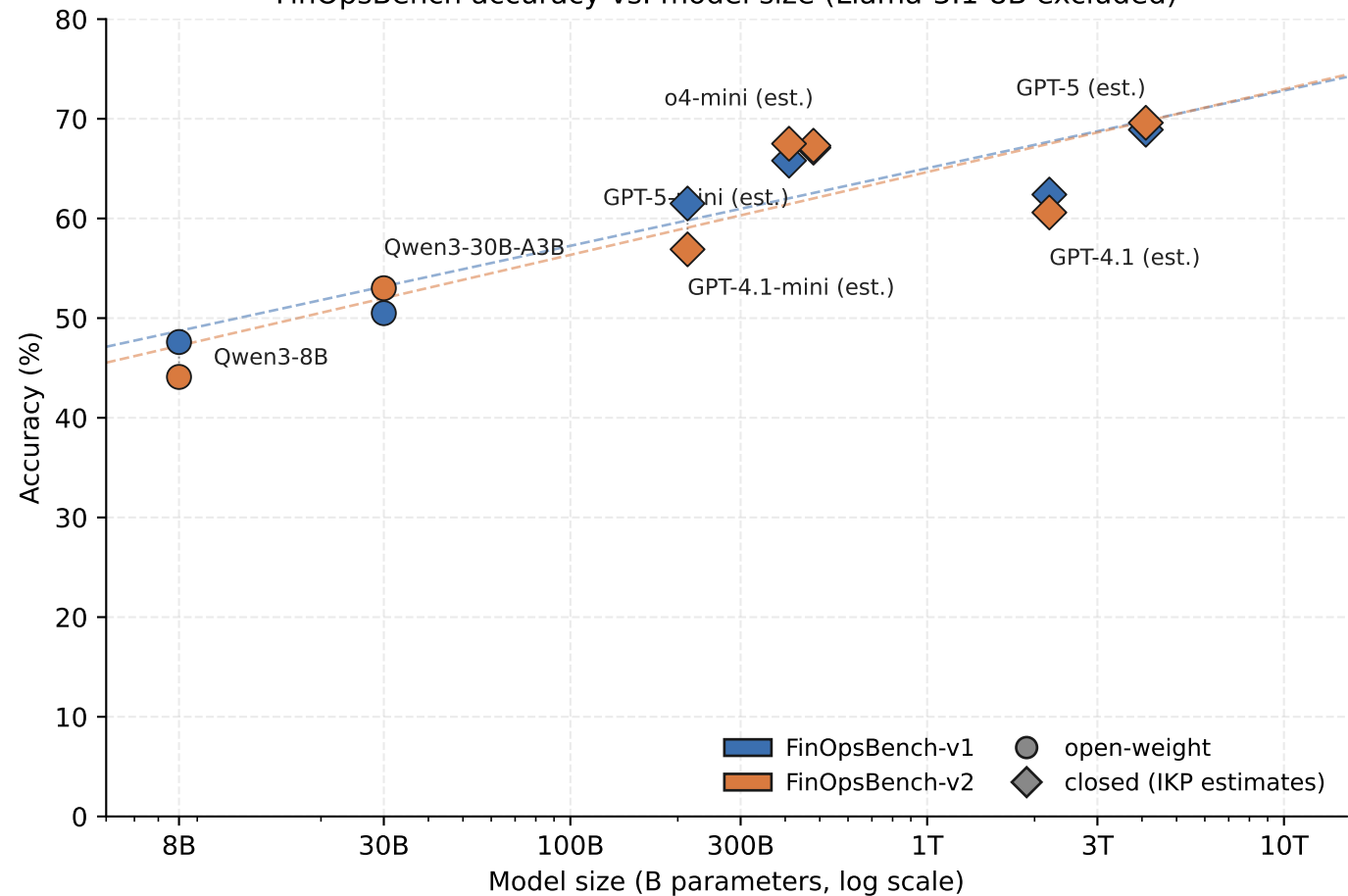
FinOpsBench accuracy vs. model size (Llama-3.1-8B excluded)
