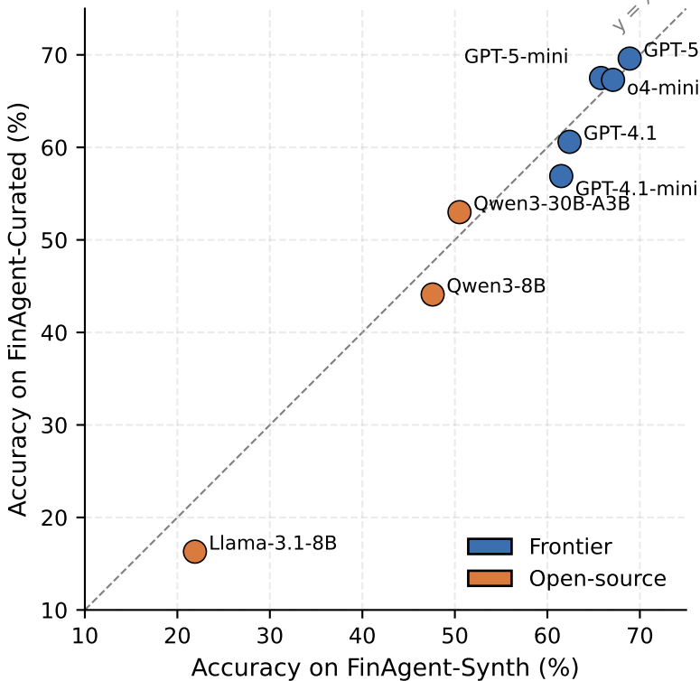
Per-model agreement between the two benchmarks
