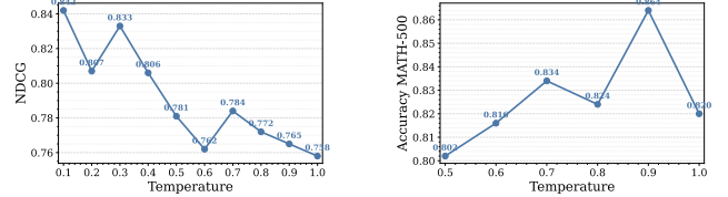
(a) Judgment NDCG@7 vs. temperature
