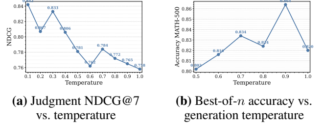
Figure 8: Temperature ablations on MATH-500 (Qwen3-8B): (a) low judgment temperature improves ranking quality (NDCG@7); (b) generation benefits from high temperature ( \sim 0.9 ) to increase solution discovery, suggesting strict judging with exploratory generation.
