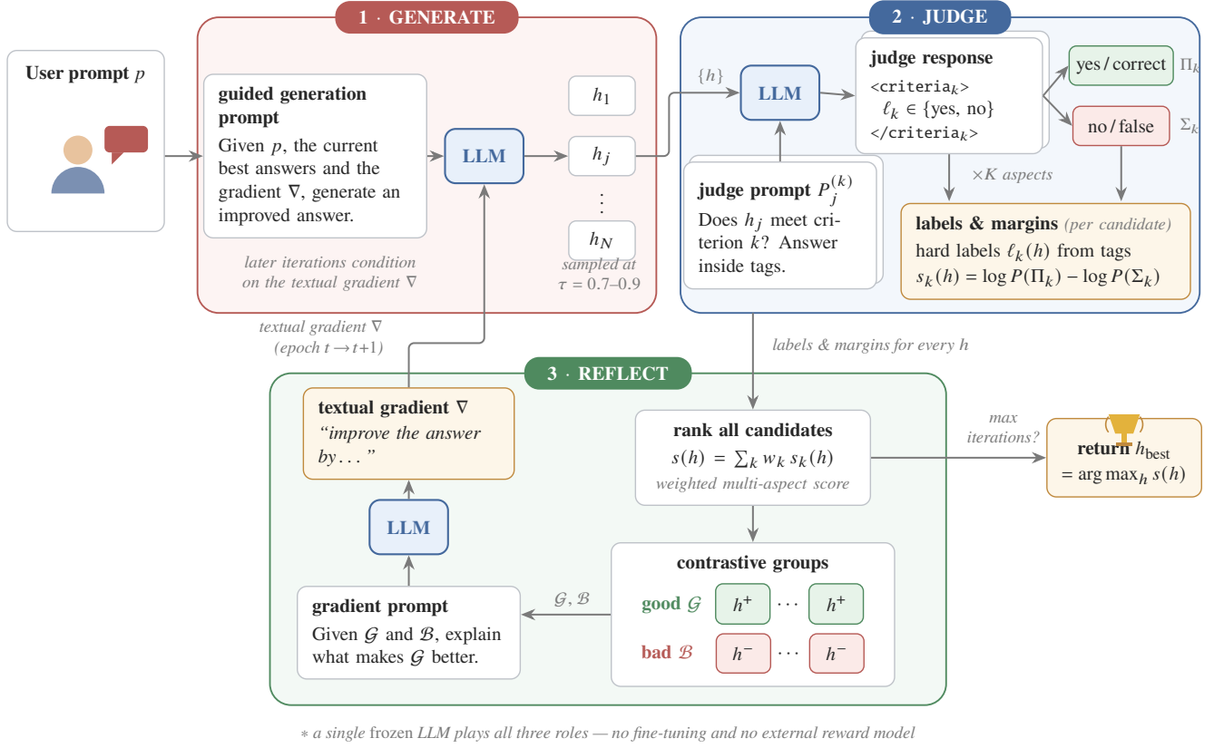
Figure 2: The SAGE framework: a single LLM acts as generator, self-judge, and reflector. Candidates are scored with contrastive label margins, partitioned into good and bad groups, and a textual gradient \nabla extracted from the groups guides the next generation round.
