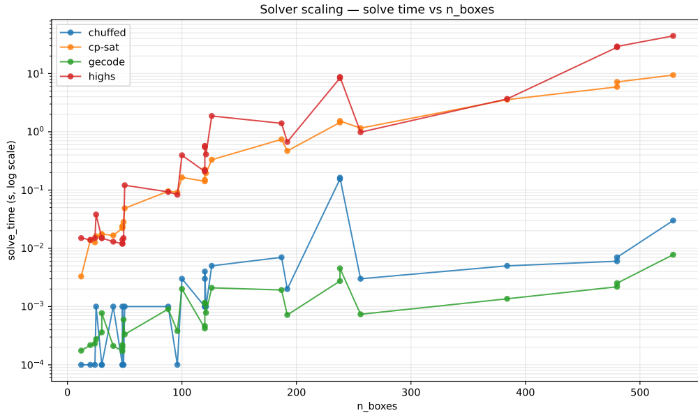
Figure 4: Solve time vs. total number of boxes — all solvers, all instances. Log scale on the time axis.
