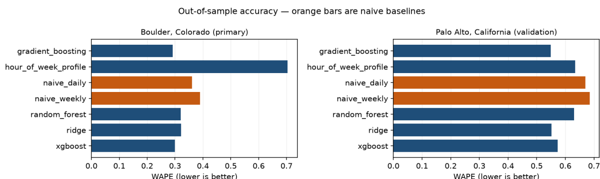
Figure 3: Out-of-sample WAPE by model. Orange bars mark the naive baselines used as the comparison floor.
