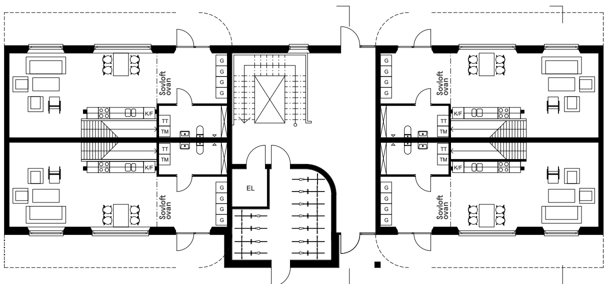
Plan 0, princip alt. 2 — Bostäder
