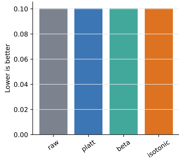
Brier score
