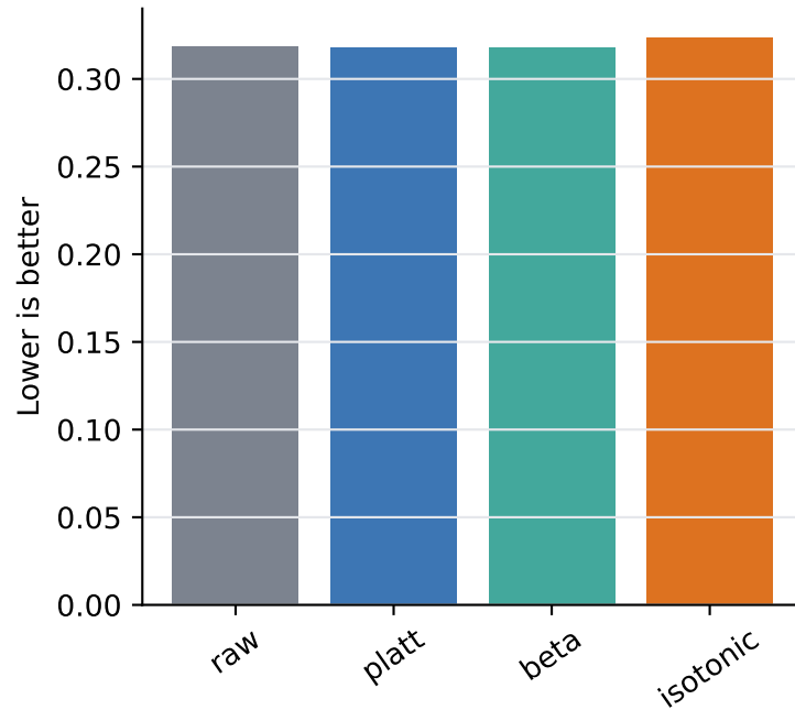
Log loss
