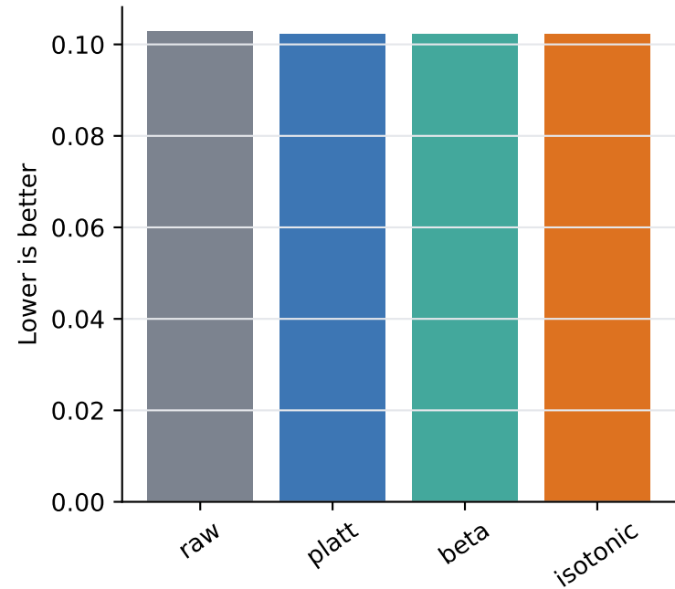
Brier score
