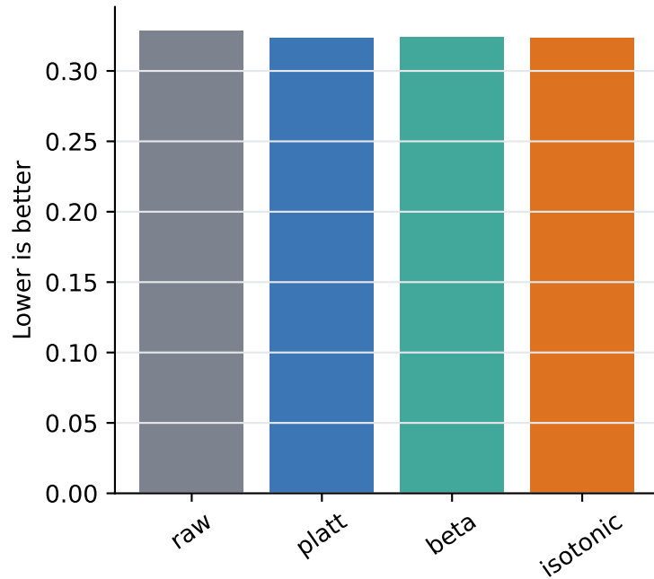
Log loss
