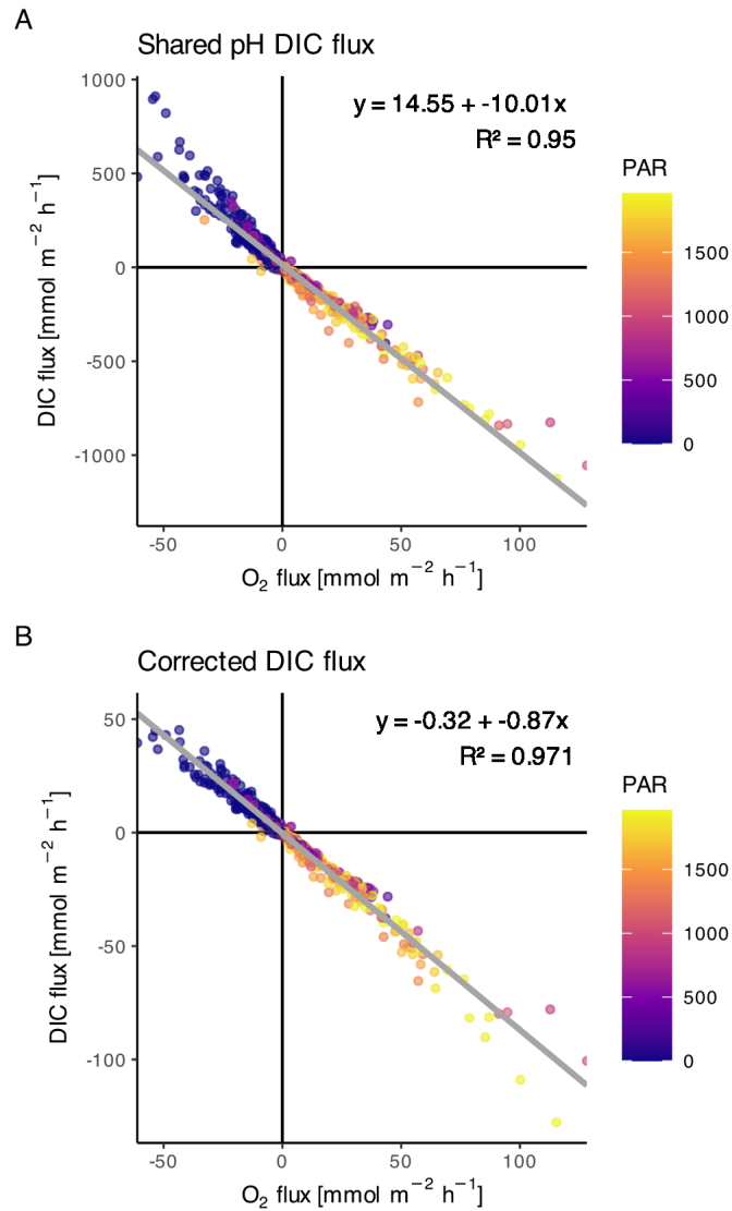
Figure 23: GEMS DIC flux relationship to oxygen flux. DIC flux is determined for the period of the SeapHOx codeployment, using measured seapHOx pH and calibrated GEMS CO 2 . The shared pH plot (A) assumes uniform pH between top and bottom inlets. The corrected DIC flux (B) holds high-inlet alkalinity constant and predicts low-inlet DIC from low-inlet CO 2 .
