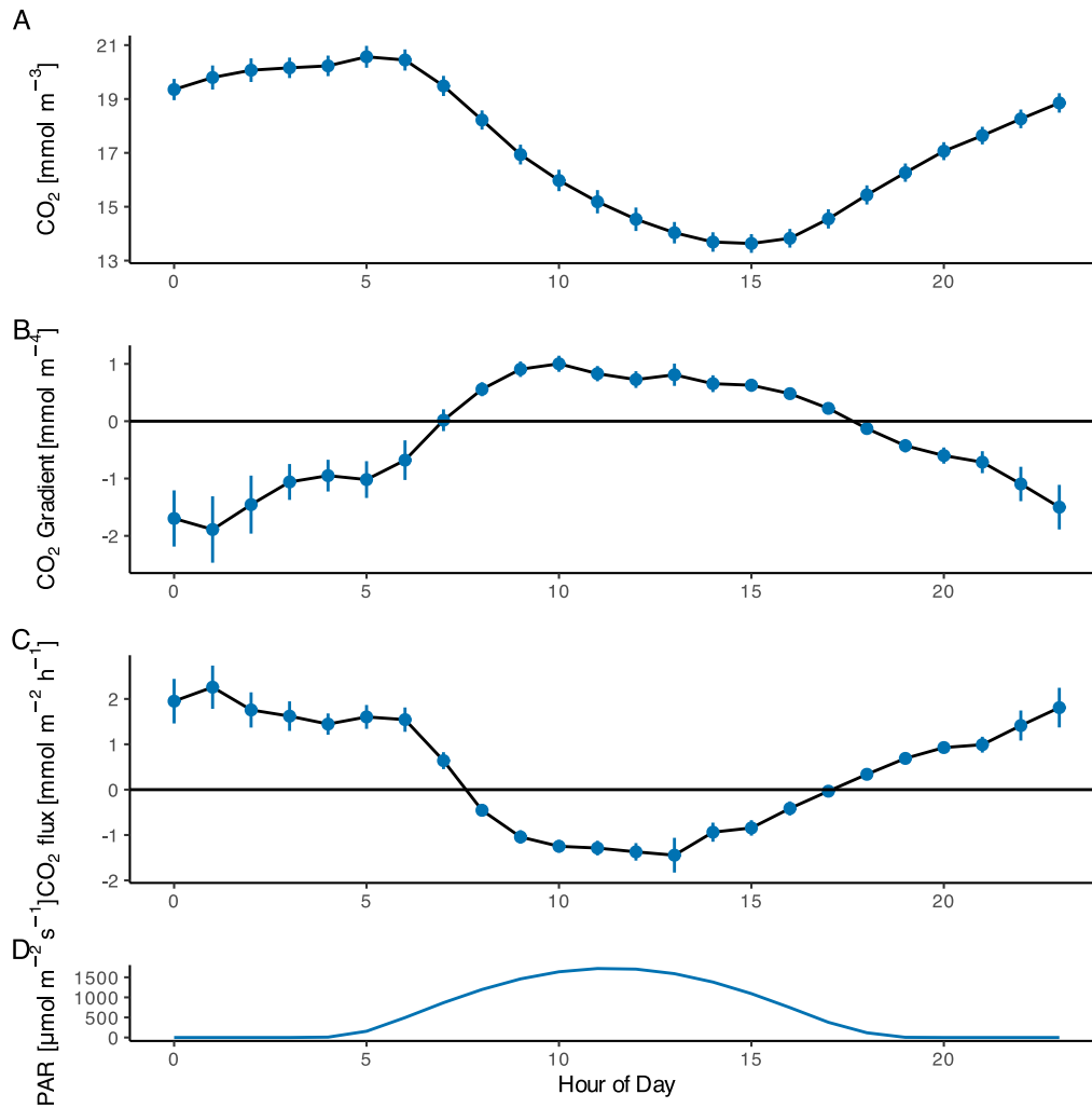
Figure 21: GEMS carbon dioxide concentration (A) and gradient (B) and flux (C) aggregated across the deployment by hour of day. Hour is adjusted to the mean solar noon for the deployment, and predicted PAR is shown in (D). CO 2 concentration is the mean across both inlets. Gradient is estimated using the difference between high and low inlets over the difference in inlet height.
