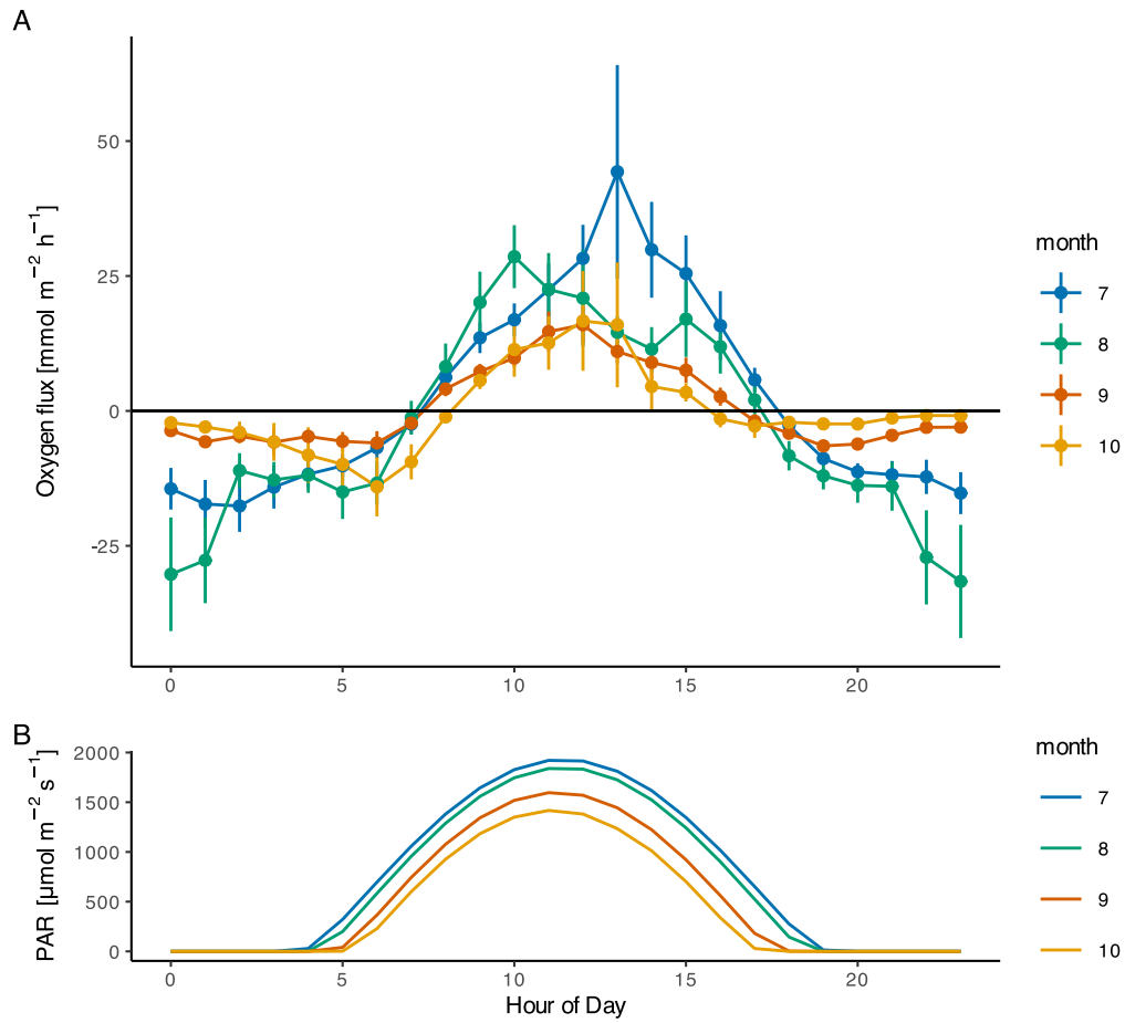
Figure 25: GEMS oxygen flux (A) and predicted PAR (B) aggregated hourly and separated by month. Hour is adjusted to the mean solar noon for the deployment. June data is not shown due to bias from only 3 days of data acquisition.
