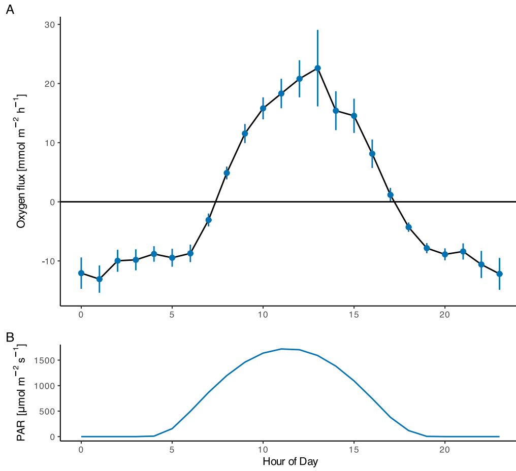
Figure 20: GEMS oxygen flux (A) and predicted PAR (B) aggregated hourly for the duration of the deployment. Hour is adjusted to the mean solar noon for the deployment.
