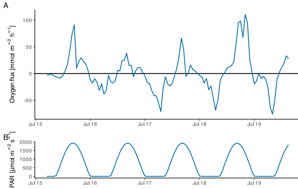
Figure 18: Oxygen flux (A) with predicted PAR (B) for comparison for the period July 15-20. Upward flux aligns with peak daily light. Respiration flux increases through the dark hours. Fluxes have strong daily variability.
