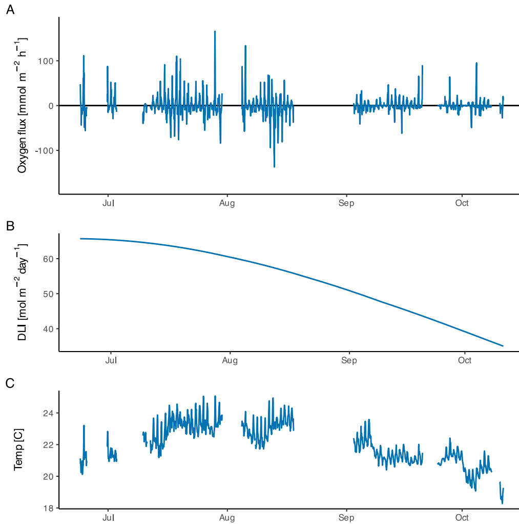
Figure 17: Hourly oxygen flux (A) for the duration of the deployment. Maintenance periods and times when the data were known to be poor due to system issues have been removed. estimated daily light integral (DLI, B) and seawater temperature at mid height (C) for comparison. Flux decreases with decreasing light and temperature. No light sensor was codeployed with GEMS, therefore photosynthetically active radiation (PAR) and DLI are estimated from modeled, cloud-free insolation. A high flux outlier on July 19 believed to be caused by fouling was removed from the plot.
