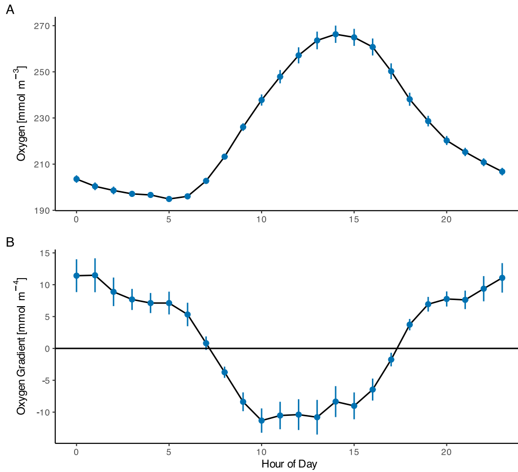
Figure 19: GEMS oxygen concentration (A) and gradient (B) aggregated across the deployment by hour of day. Hour is adjusted to the mean solar noon for the deployment. Oxygen concentration is the mean across both inlets. Gradient is estimated using the difference between high and low inlets over the difference in inlet height.
