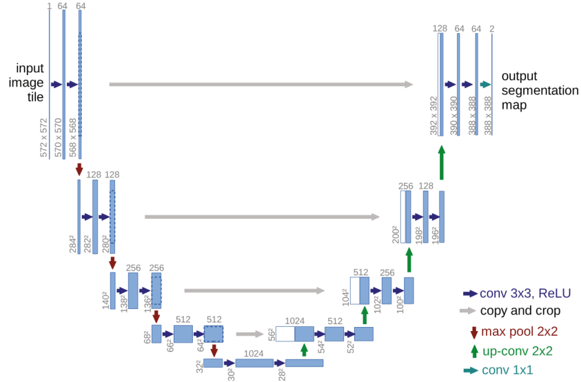
Figure 5-1 Original U-NET architecture from [Ronneberger et al., 2015].
