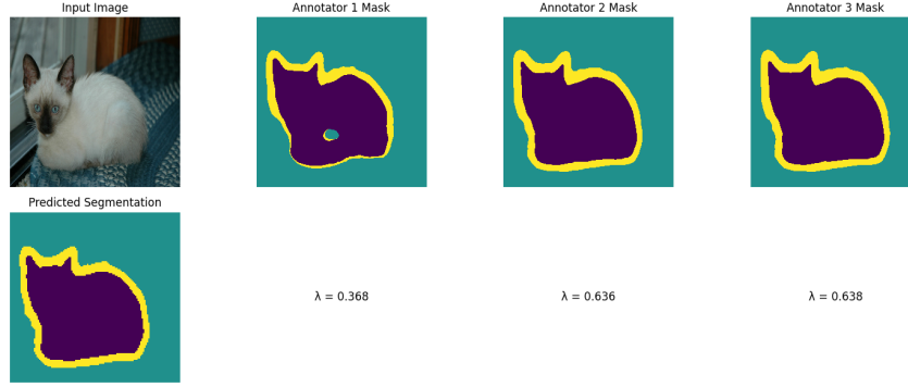
Figure 5-9 Example evaluation of the proposed model in its last trained epoch. An accurate segmentation output is delivered as well as scalar reliability estimations from the labelers masks. Disturbance signal-to-noise ratios are: [-20, 0, 10] dB from left to right. Best found hyperparameters: learning rate = 0.0011, q = 0.4 , noise tolerance = 0.2, \alpha_{reg} = 0.26 , \alpha_{entropy} = 0.03 , \alpha_{sum} = 0.27 .
