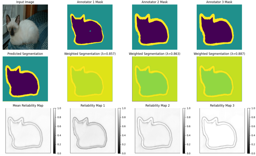
Figure 5-10 Example evaluation of the proposed model in some given epoch (15/50) of training, which demonstrates a quick convergence of the model for correctly estimating the reliability of the labelers masks. An accurate segmentation output is delivered as well as pixel-wise reliability estimations from the labelers masks. Disturbance signal-to-noise ratios are: [-20, 0, 10] dB from left to right. learning rate = 0.00065, q = 0.66 , \tilde{C} = 0.64 , \alpha_{centroid} = 3.6 , \alpha_{entropy} = 2.3 , \alpha_{\lambda} = 1.7 , \beta = 0.77 .
