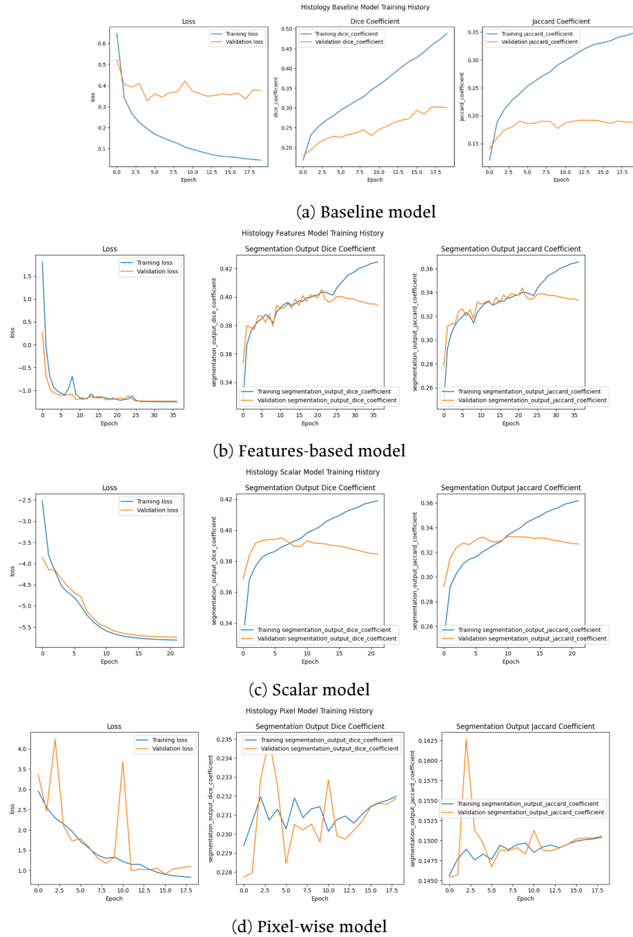
Figure 5-17 Training curves comparison for different model variants on the TNBC (Crowd-Seg) dataset: (a) baseline model, (b) features-based model, (c) scalar model, and (d) pixel-wise model.
