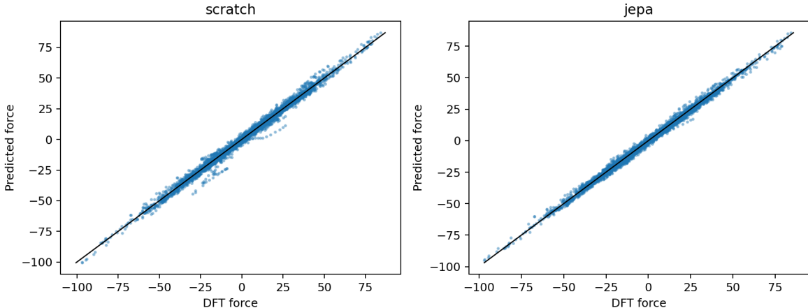
Figure 1: Force prediction scatter for scratch and JEPA-initialized models. Predicted force components are plotted against DFT reference force components for the held-out MD17 ethanol test split. The diagonal line indicates perfect agreement. The JEPA-initialized model exhibits a lower force RMSE than the scratch baseline after the same number of supervised epochs.
