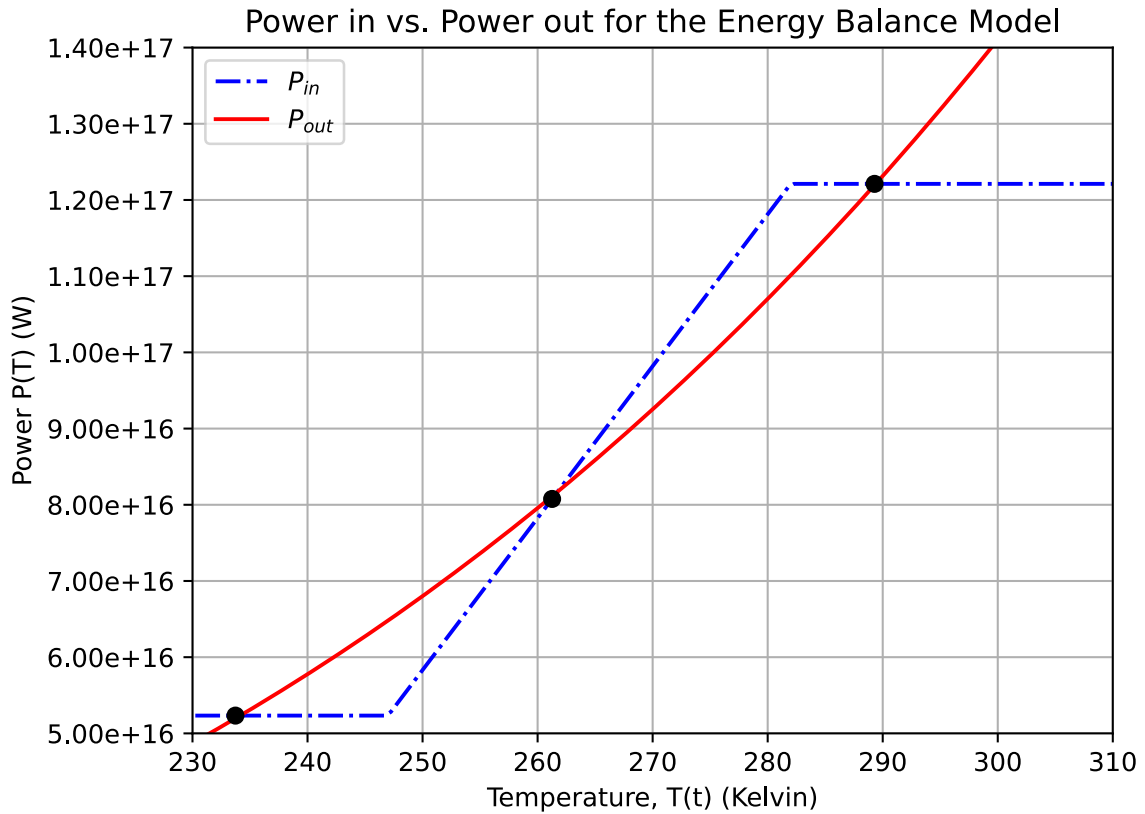
Figure 2: A graph of the power flowing into and out of the earth at different surface temperatures. The dots represent the temperatures and powers where P_{in} = P_{out} (i.e the intersection points of these lines).
