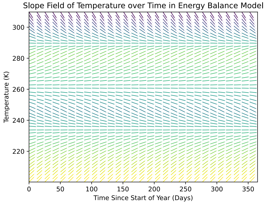
Figure 4: The slope field of surface temperature over time predicted by the EBM. The lines represent the slope of the tangent line of a possible temperature curve at that point. The lines are normalized to be a standard length, and colored based on their slope. See Appendix B, for the code to generate this graph.
