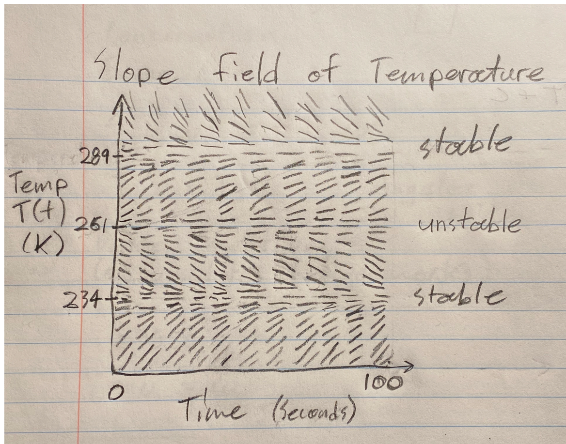
Figure 5: Just in case, I also drew the slope field by hand. I am a computer guy, not a drawing guy. The image shows how the slope lines point away from the unstable equilibrium at T = 261.26K , and towards the stable equilibriums at T = 289.29K and T = 233.73K over time.
