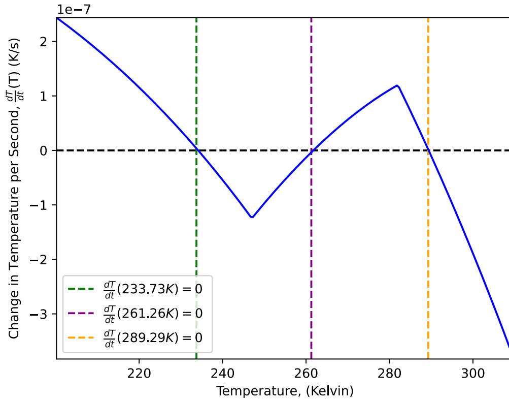
Figure 3: The change in temperature per second predicted by the EBM at different surface temperatures. This shows that at 234K, 261K, and 289K the change in temperature over time is zero - highlighted by the dashed lines intersecting the derivative line and zero line. See Appendix C, for the code to generate this graph.
