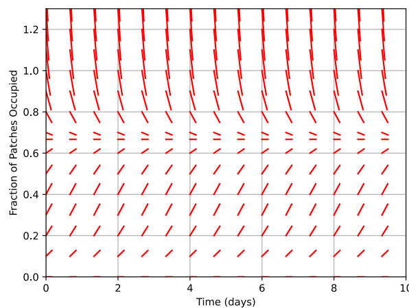
Figure 1: A slope field of the fraction of inhabited patches over time showing an unstable equilibrium at p = 0 and stable equilibrium at p = \frac{2}{3} is a stable equilibrium
