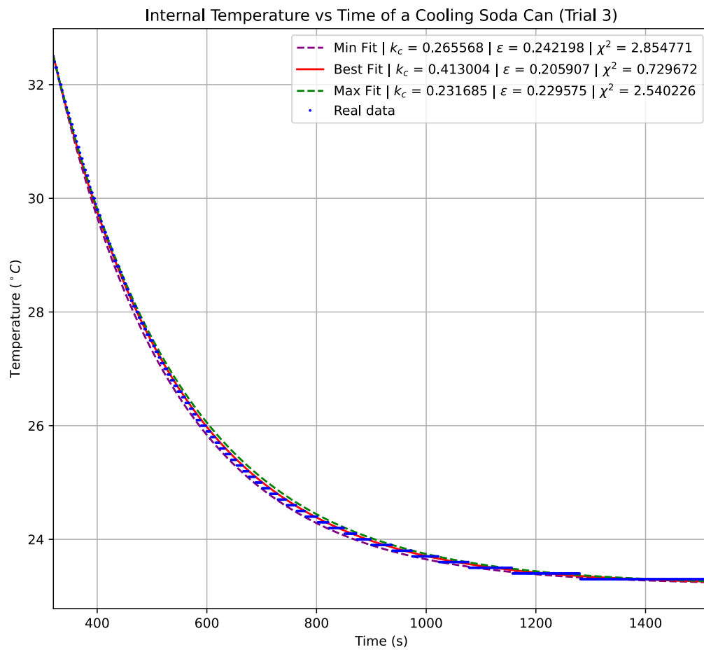
Figure 4: Graph of the internal temperature over time for Trial 3.
