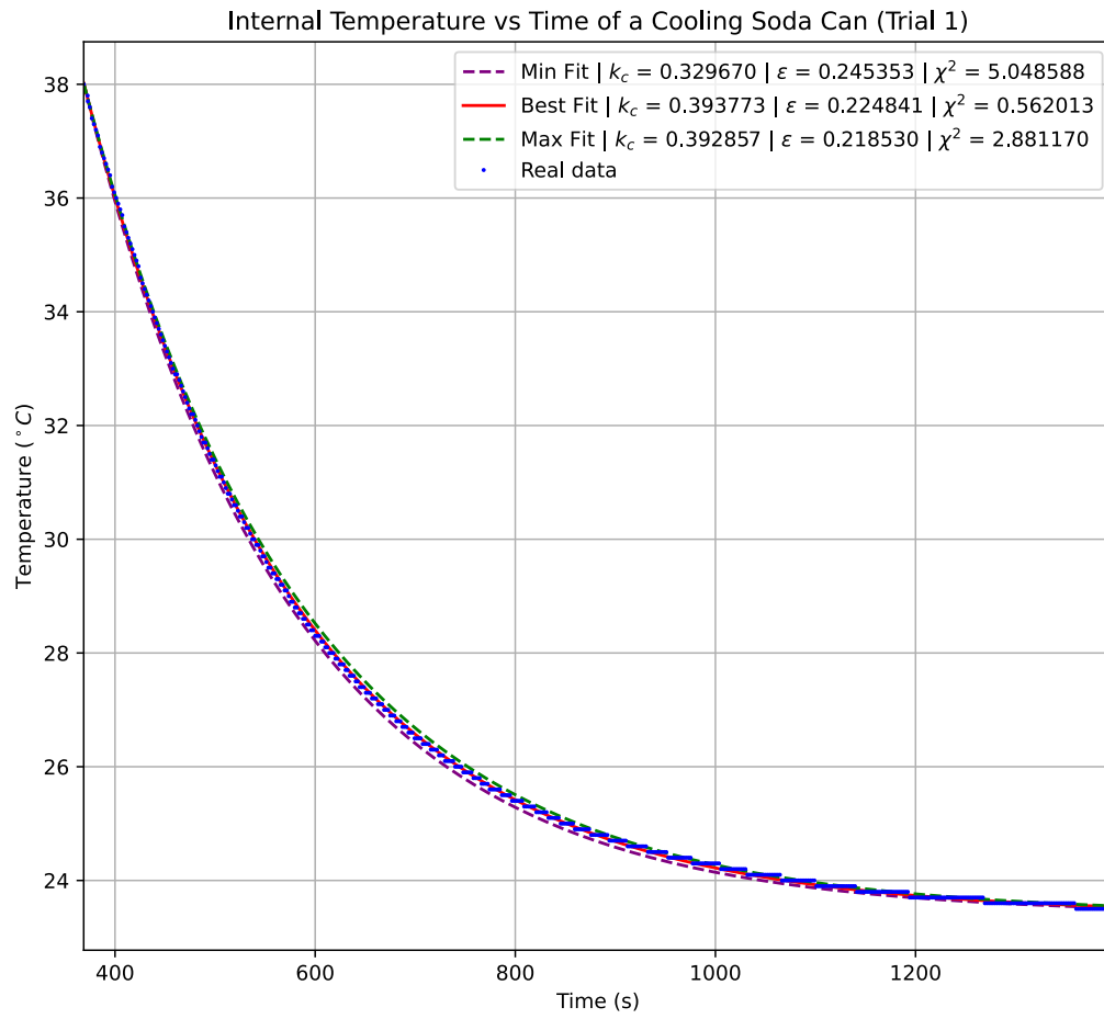
Figure 6: Graph of the internal temperature over time for Trial 1.
