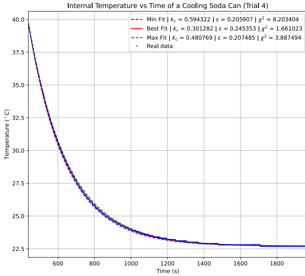
Figure 5: Graph of the internal temperature over time for Trial 4.
