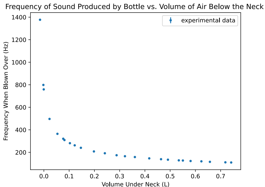
Figure 4: Plot of frequency produced by the bottle when blowing over the neck vs. the volume in the bottle under the neck (in the body). Note that error bars are included, however the error is too small to be shown outside the size of the dots. This is true for all of the following graphs.
