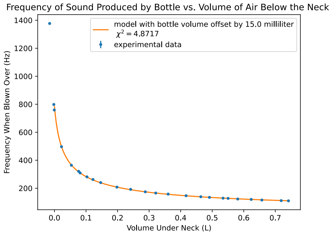
Figure 7: Plot of frequency produced vs. the volume in the bottle under the neck. The volume of air under the neck is reduced by 15 ml before the model is applied.
