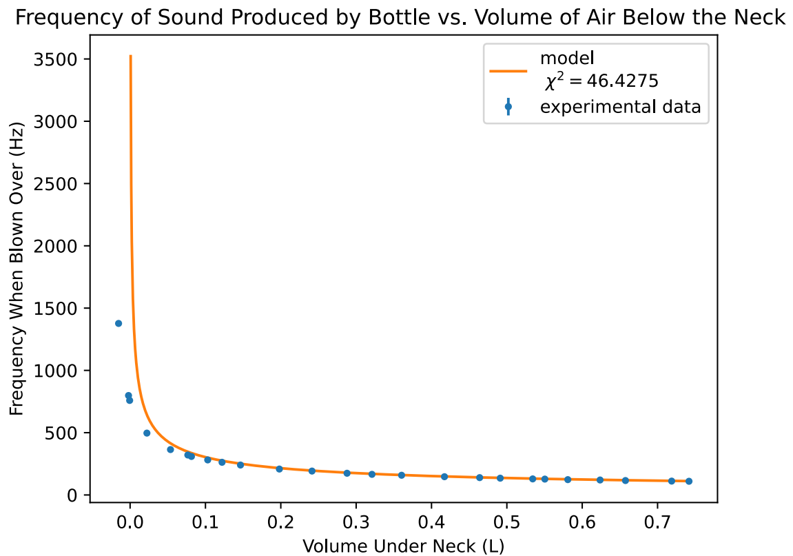
Figure 5: Plot of frequency produced by the bottle when blowing over the neck vs. the volume in the bottle under the neck (in the body) with a line representing the model.
