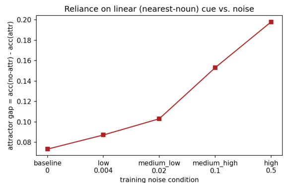
Figure 3: Attractor gap (no-attractor minus attractor accuracy) vs. noise rate. The monotonic rise indicates increasing reliance on the linear cue.
