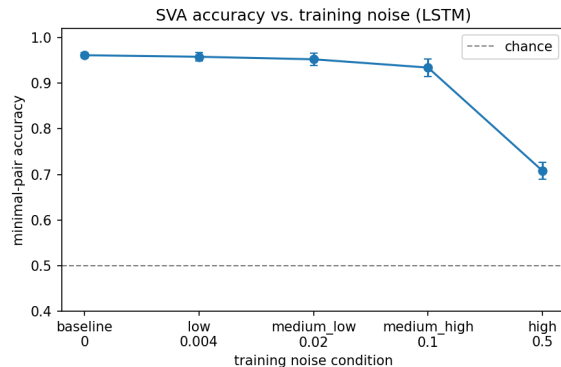
Figure 1: Overall minimal-pair accuracy vs. injected SVA noise rate. The dashed line marks chance (0.5). Performance is flat through 10% noise and falls sharply at 50%.
