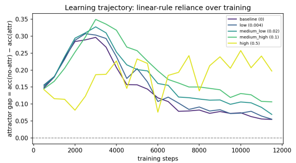
Figure 7: Attractor gap over training steps, one curve per noise condition.
