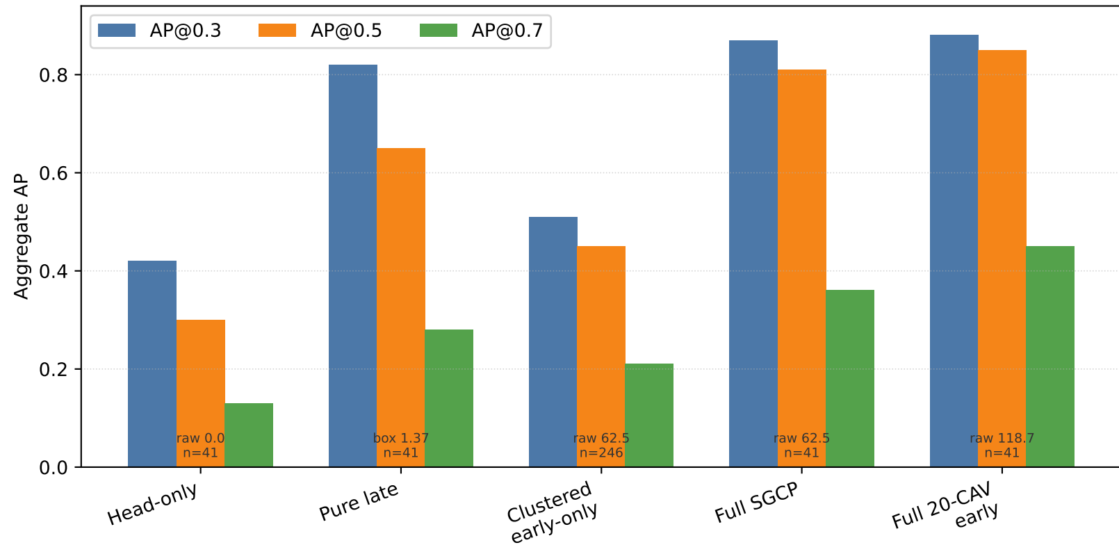
Attentive Fusion Contribution by IoU Threshold
