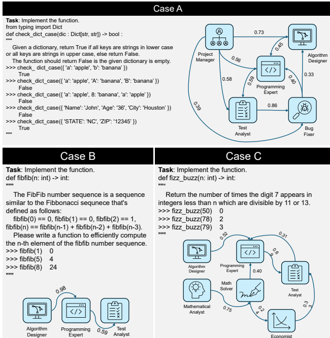
Figure A3: Further case study for code generation tasks, grouped by how the optimal agent set compares to a hand-designed “intuitive” roster: fully-intuitive , partially-intuitive , and counter-intuitive .
