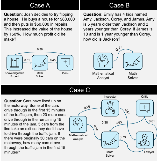
Figure A2: Further case study for mathematical reasoning tasks, grouped by how the optimal agent set compares to a hand-designed “intuitive” roster: fully-intuitive , partially-intuitive , and counter-intuitive .
