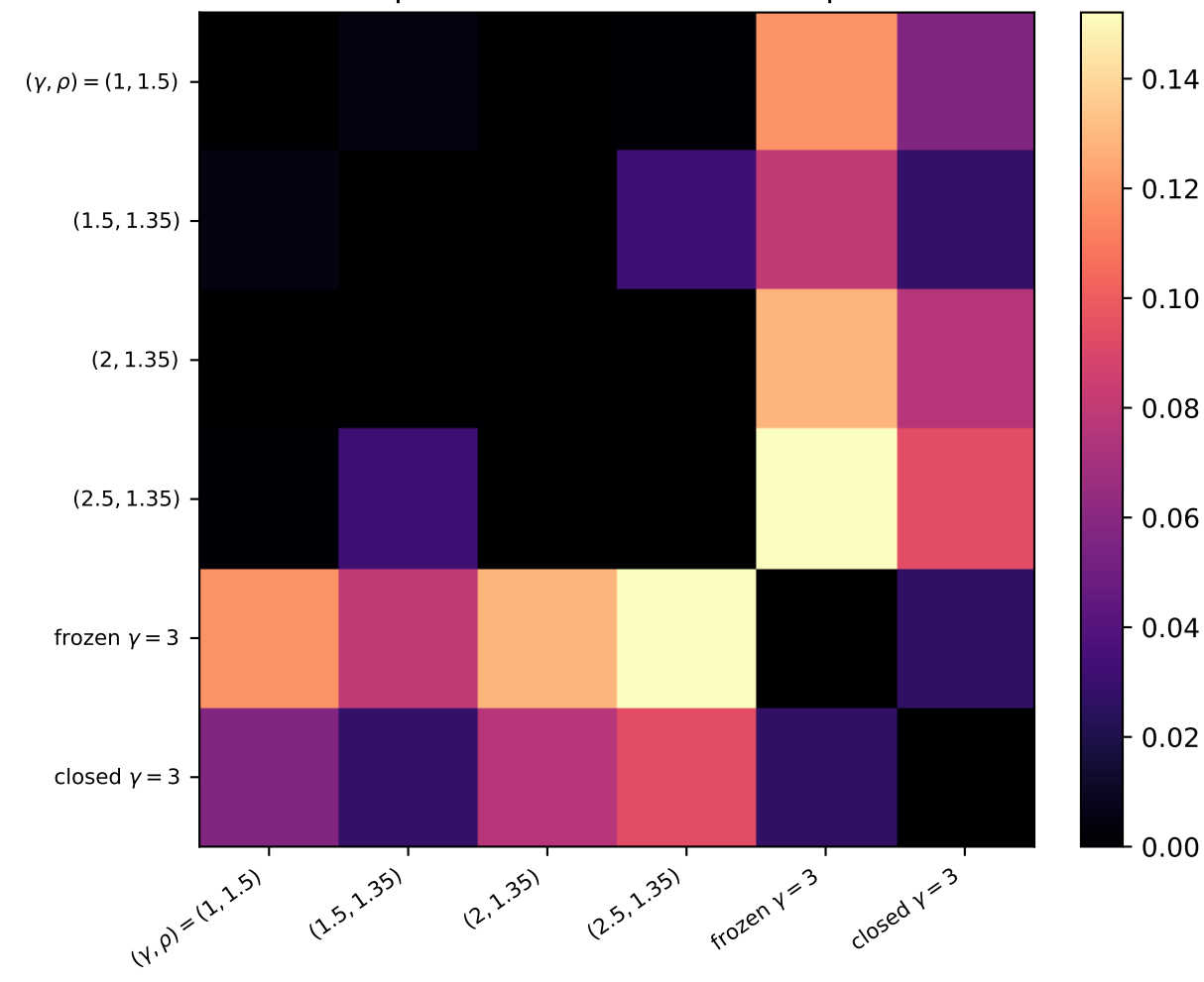
D. Endpoint feature C2ST above split-null
