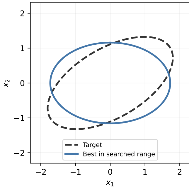
Guidance: tune scale only
