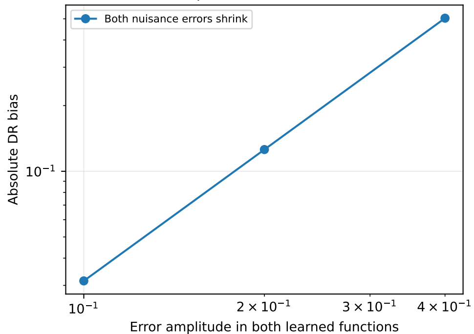
Bias is a product of nuisance errors
