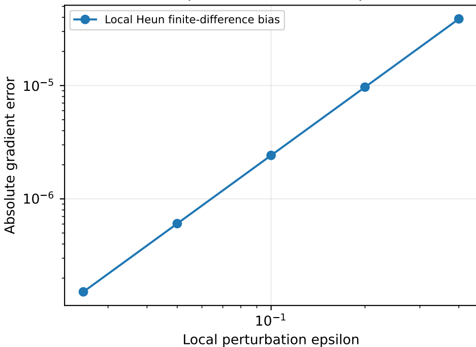
Finite-step derivative error is quadratic
