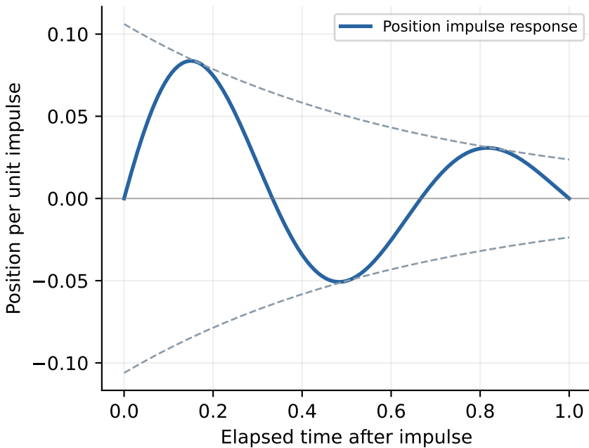
Stable plant: decaying response
