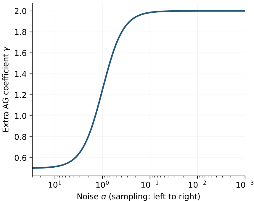
Exact Gaussian denoiser correction
