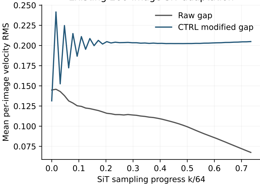
Existing 200-image SiT adaptation
