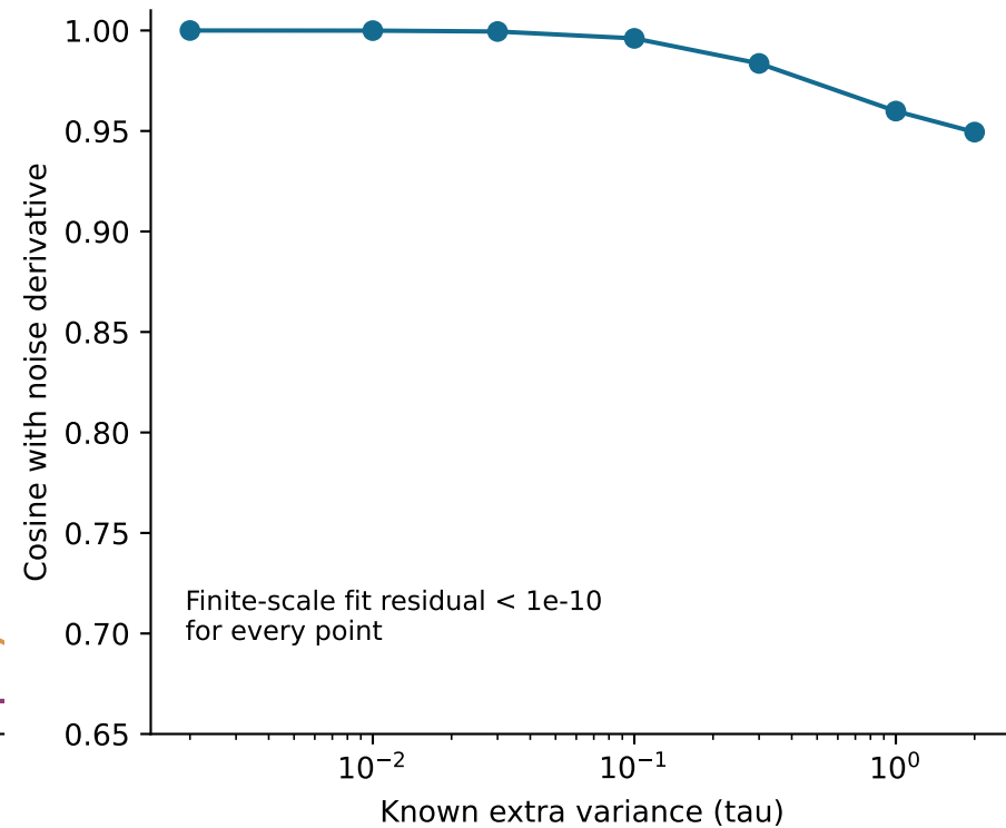
B. Exact heat family need not be collinear
