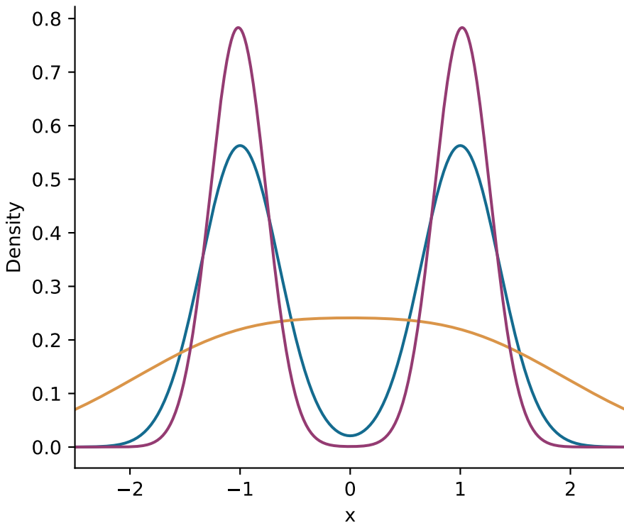
A. Heat smoothing can join two modes
