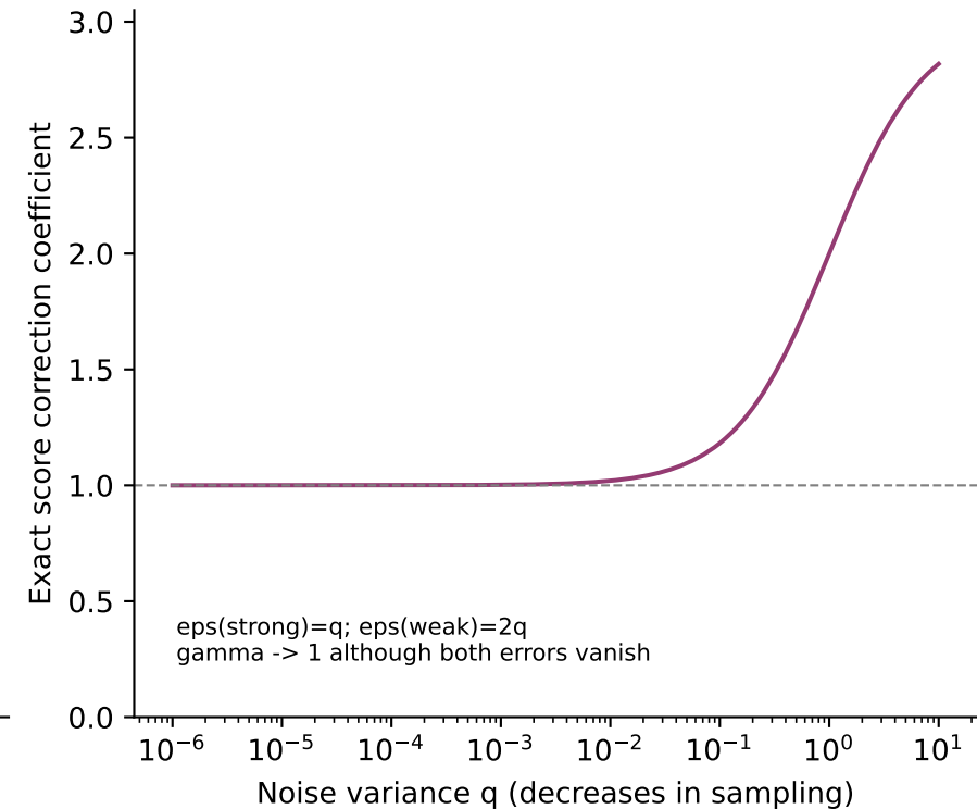
C. Low-noise coefficient need not vanish
