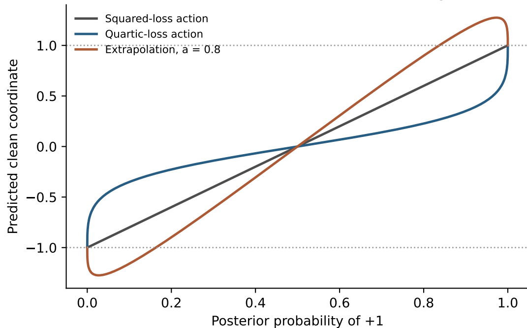
Two candidates: exact odds flattening
