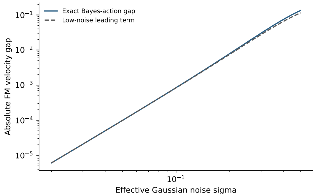
Smooth prior: gap vanishes at low noise
